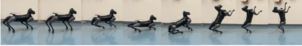
Figure 7: Skill Transitioning: Hop to Stand on Bare Floor
