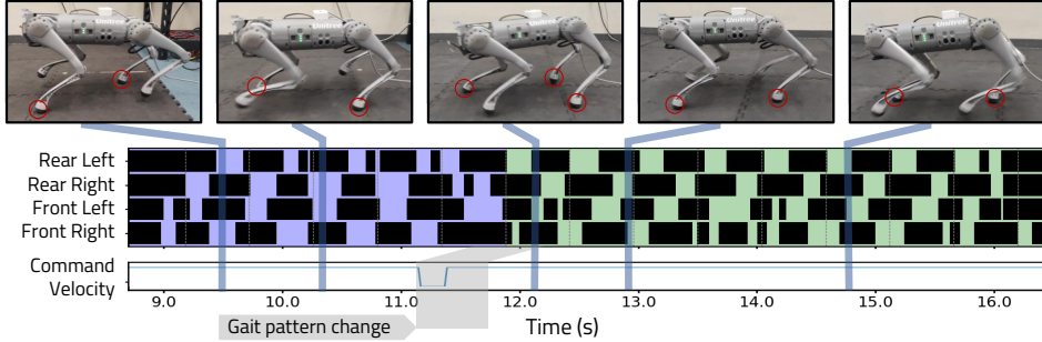
Figure 4: Demonstration of stable walking with different modalities. The red circle denotes the legs in contact with the ground. The robot initially walks using trotting skill, shown in purple background, then switches to pacing, shown in green, following a command change that involves a sudden stop and resume. We emphasize DiffuseLoco’s ability to maintain different modalities under the same command, switching only when necessary.
