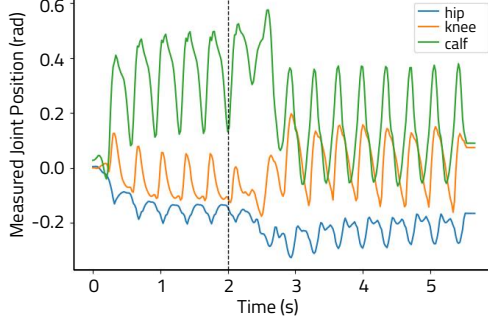
Figure 13: Joint positions during transition from hopping to pacing. The vertical dashed line marks the time of receiving the pacing command.
