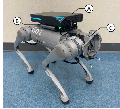
Figure 17: Onboard compute experiment setup. A: Mini computer with Intel Core i7-13700H and NVIDIA GeForce RTX 4060 Mobile. B: Battery bank. C: Go1 quadrupedal robot. This setup is within the robot’s load capacity, enabling real-time deployment of our diffusion model using the acceleration framework.
