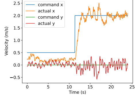
Figure 14: Bipedal robot skill transitioning. Velocity tracking with transition from walking to running on the bipedal robot Cassie in Mujoco simulation.
