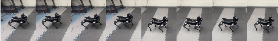
Figure 12: Skill Transitioning: Hop to Pace
