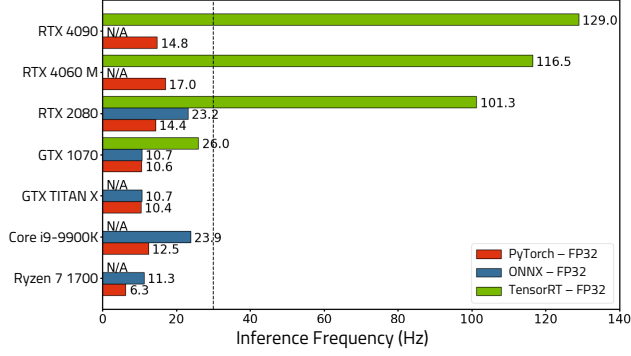
Figure 16: Benchmark of running our DiffuseLoco policy (6.8M parameters) on different hardware platforms. The dashed line marks the 30 Hz minimum frequency required for real-time robot control. TensorRT optimization achieves approximately 7x speedup compared to the naive PyTorch implementation. N/A entries reflect that the hardware is incompatible with the inference workflow.
